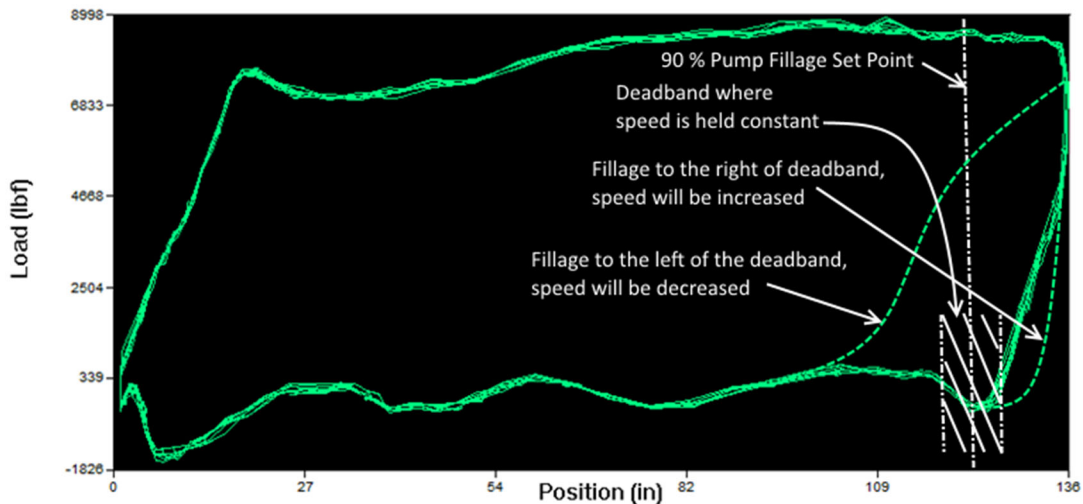
Deadband description for VFD Surface mode
