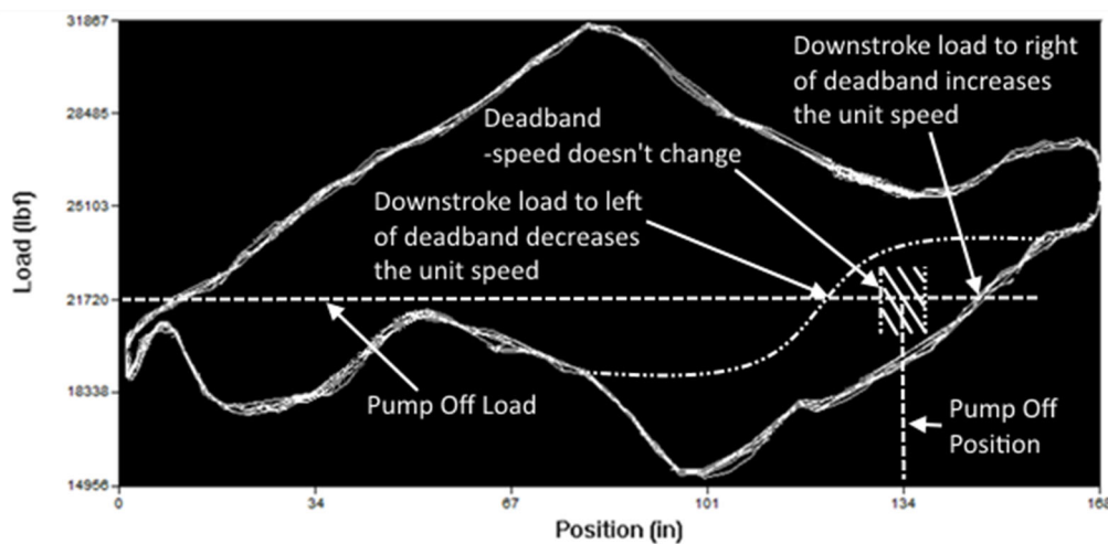
Deadband description for VFD Surface mode
