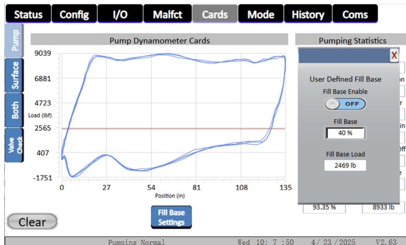
Cards - Pump - Fill Base pop-up
