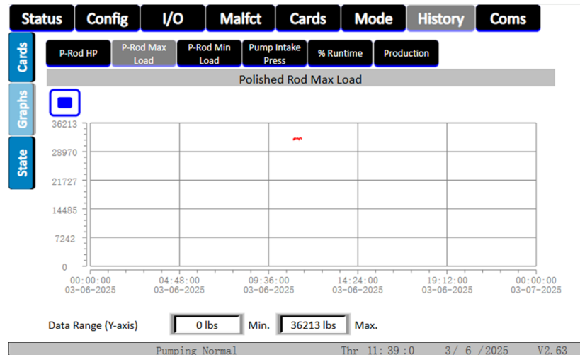
History – Graphs – Polish Rod Max Load
